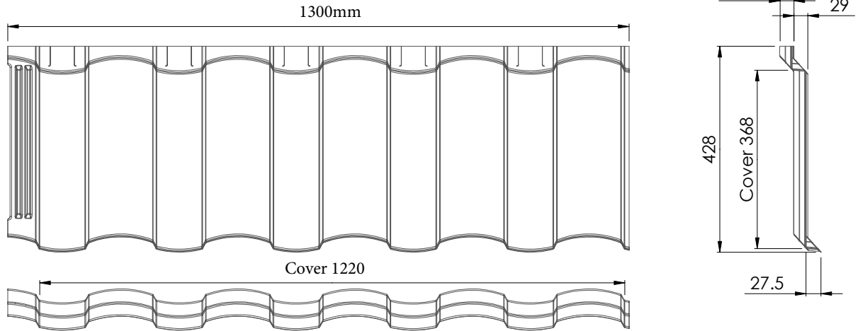
Tile Dimensions
