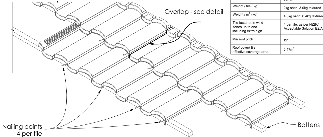
Nailing Detail
