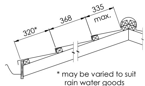
Batten Layout
