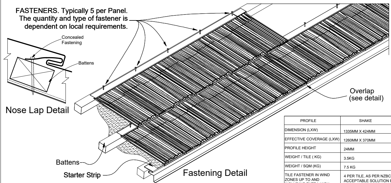
Tile Dimensions
