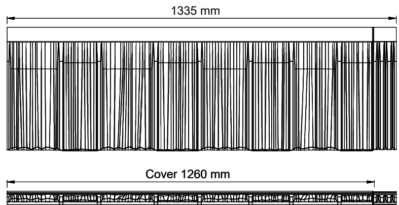
Tile Dimensions
