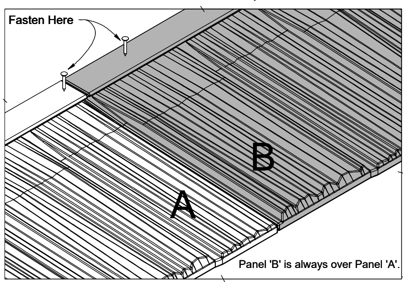
Overlap Detail
