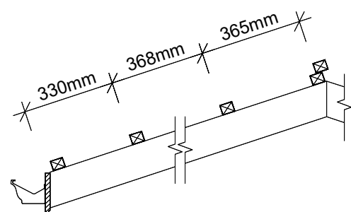
Batten Layout
