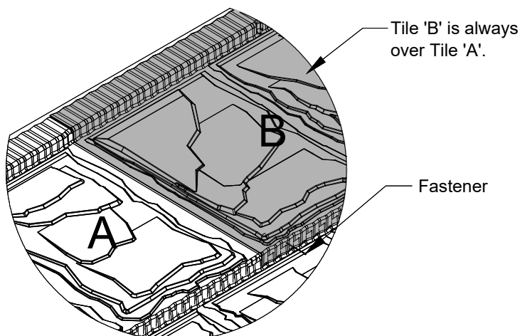
Overlap Detail
