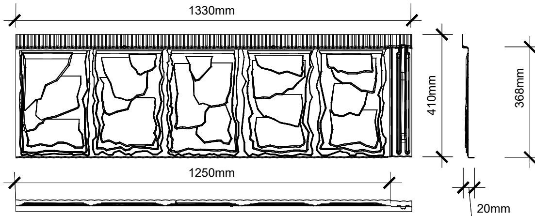
Tile Dimensions
