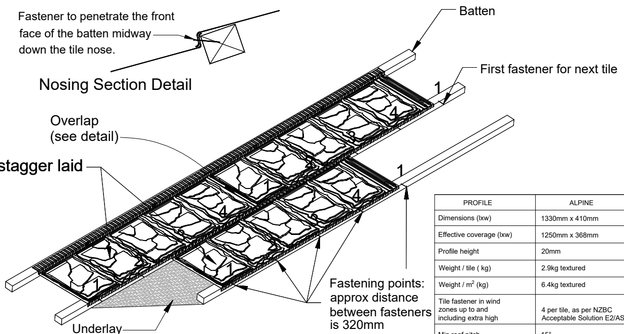
Fastening Detail
