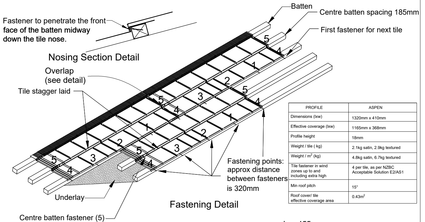
Tile Dimensions
