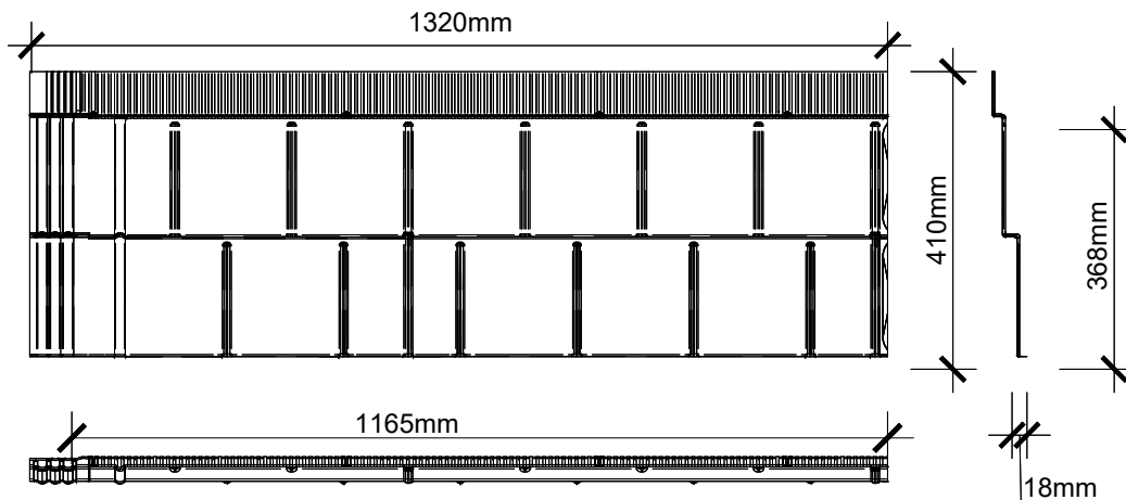
Tile Dimensions
