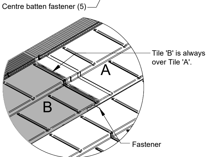
Fastening Detail
